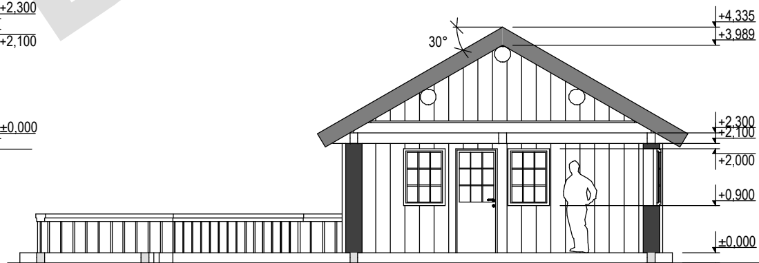
SECTION C-C
